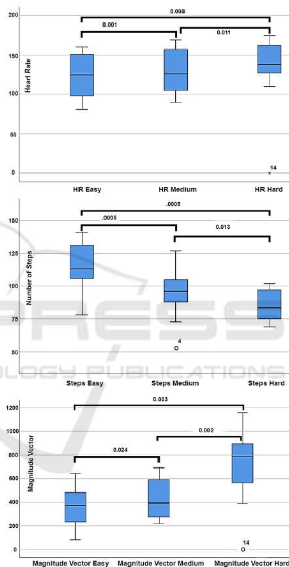
Figure 3: Boxplot from post hoc results of Heart Rate, Magnitude Vector, and number of steps.
