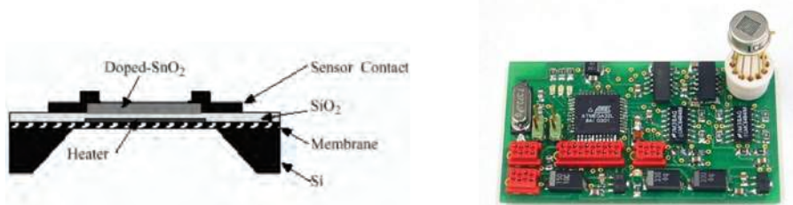
Fig. 1. The artificial nose sensor system. Left panel: schematic of each of the sensors of the 6 grid array including its main components. The size of a sensor is 0.18 x 0.2 mm (with x length), with an active area of 0.032 mm 2 . Right panel: the full chemo-sensor package and its readout PCB. The sampling frequency of the PCB is 16.3 Hz, its dimensions 60 mm x 35 mm, and its weight 13.8 g. Adapted from Pyk et al. (2006)
