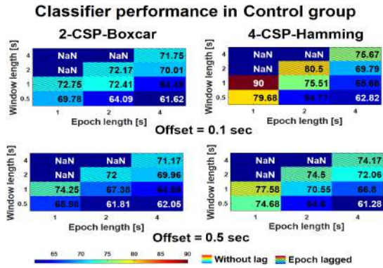
Figure 6: Classifier performance for control group (diagonal lines represent epoch-lagged configurations).
