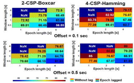
Figure 5: Classifier performance for age-matched group (diagonal lines represent epoch-lagged configurations).
