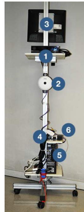
Fig. 8. The data acquisition and recording system. 1 - Kinect sensor, 2 - Fish eye camera, 3 - Computer Screen, 4 - Bluetooth receiver, 5 - PC Computer, 6 - Data Storage Hard Drive.
